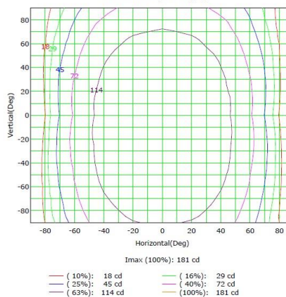
Isocandela (rectangle)
